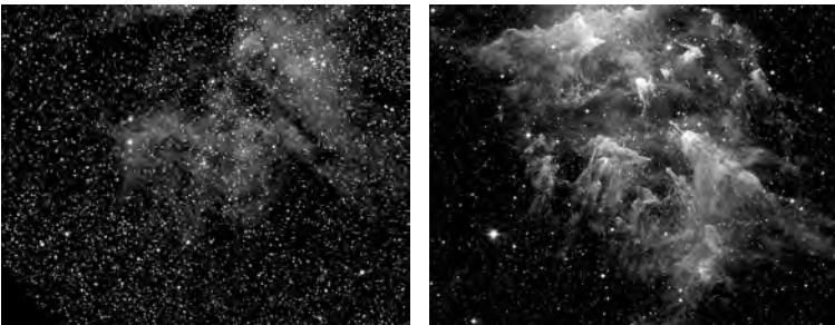
A visible-light (NOAO – left) and infrared (Spitzer – right) comparison of Eta Carinae.
